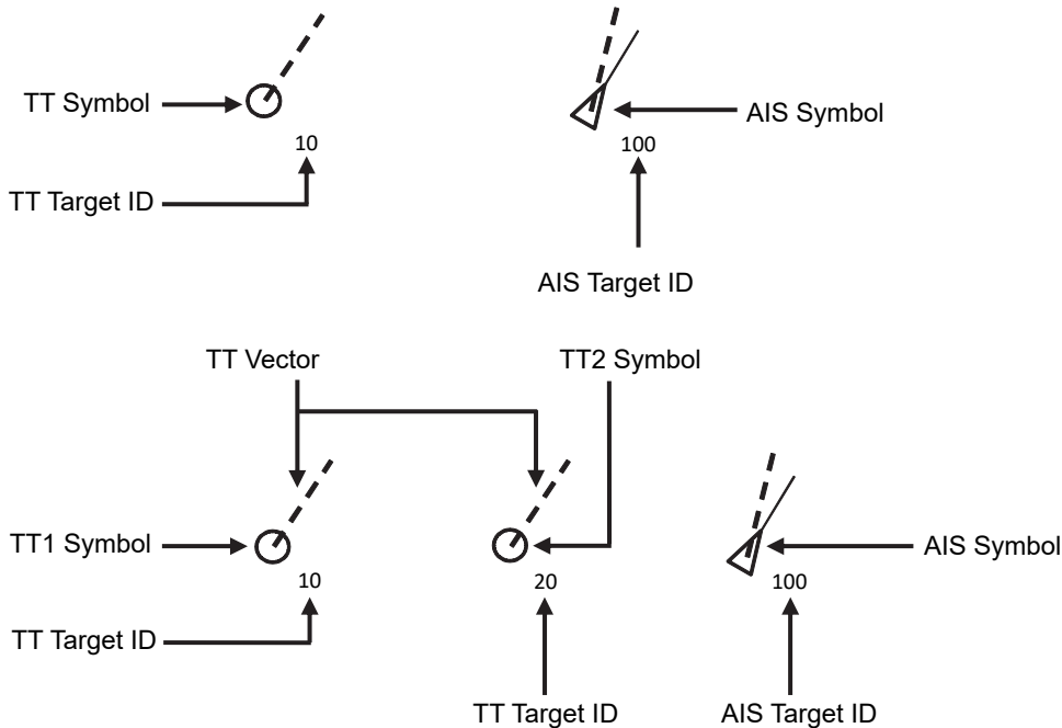
ECDIS screen
