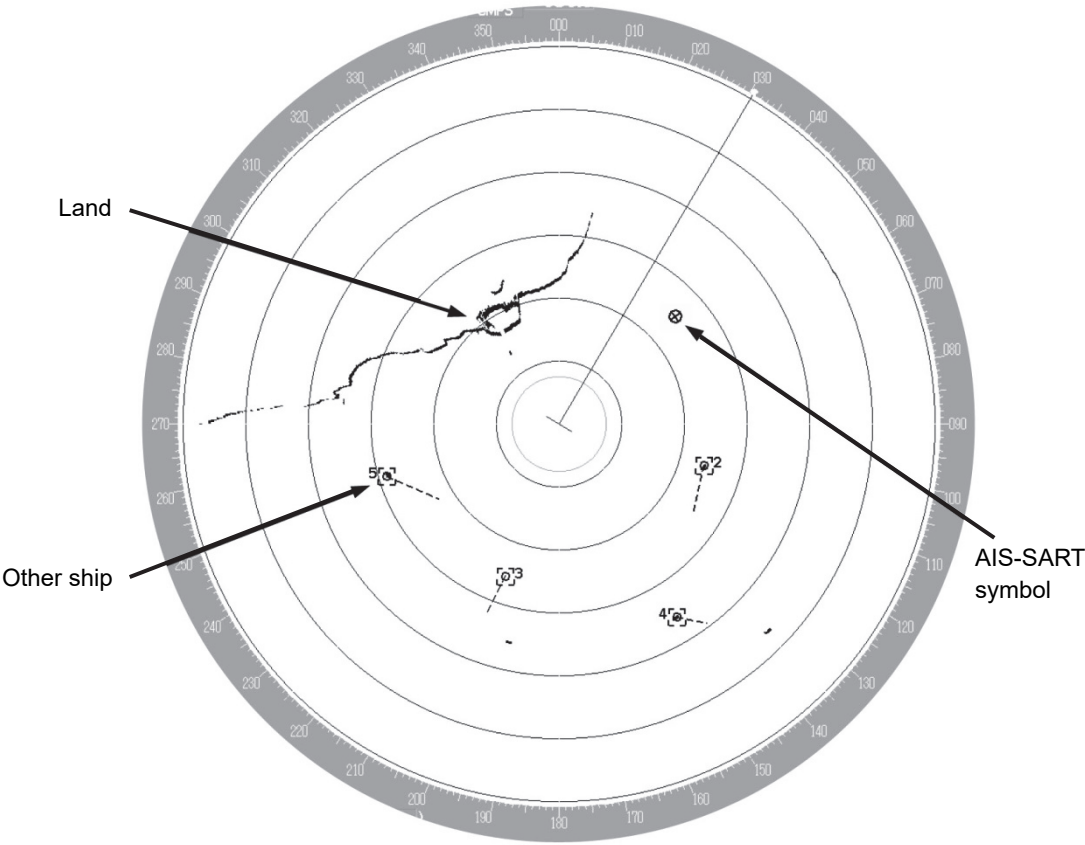
Example of AIS-SART Symbol Display
